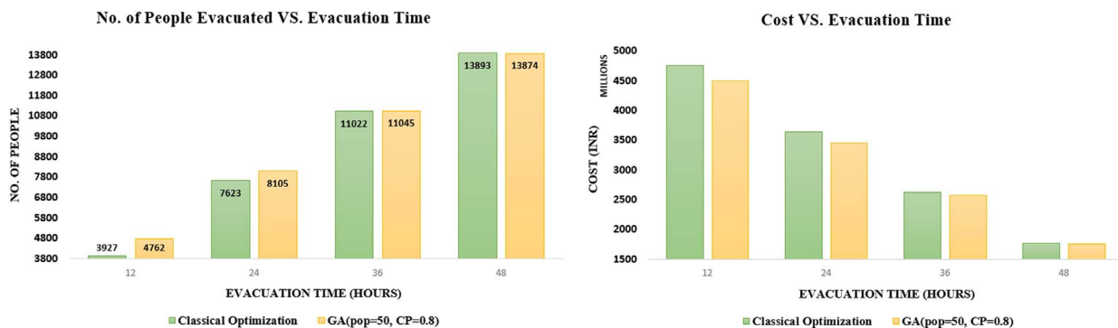
Fig. 7. No. of people evacuated vs. Evacuation Time (left) and Cost vs. Evacuation Time (right) for Classical optimization and GA for Case Study Data.
